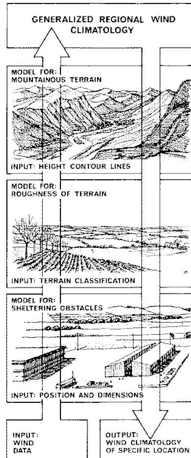
Figure 5. Wind atlas methodology of WAsP
