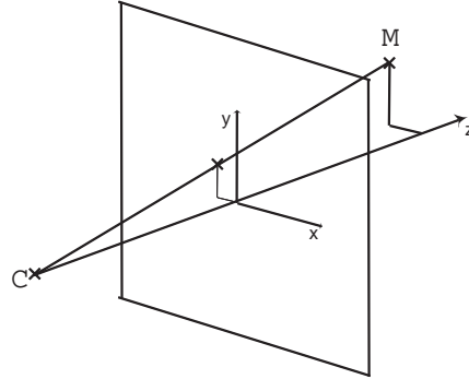
Fig. 1. Cartesian coordinates and “pinhole model”. C is the optical center, Cz the optical axis, Cx and Cy are parallel to the image plane, and (Cx, Cy, Cz) is an orthonormal frame. The point M is expressed in cartesian coordinates in the camera frame. We assume the focal length to be 1.
