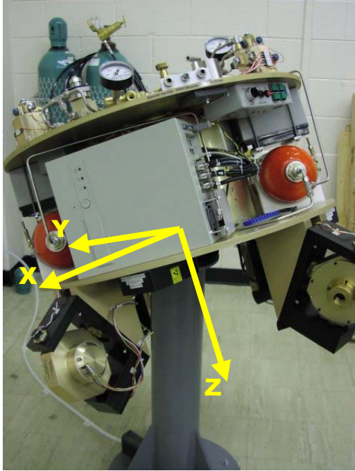
Fig. 6. The body-axes definition for the IACS. The x -axis is designated as the roll axis, the y -axis is designated as the pitch axis and the z -axis is designated as the yaw axis.
