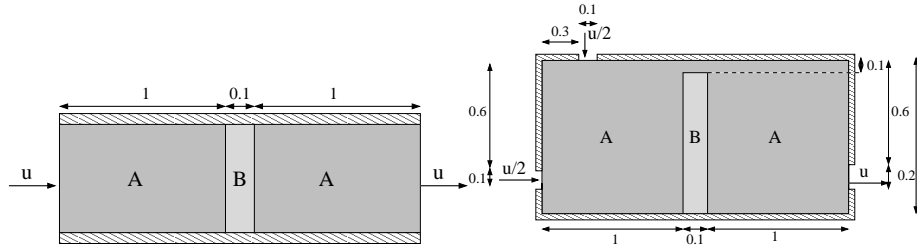
Fig. 1 Geometry of the 1D and 2D cases.
