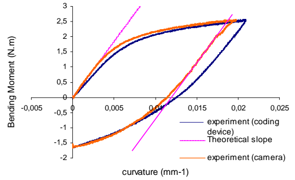
Figure 5: Moment-Curvature diagram
