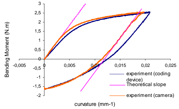
Figure 5: Moment-Curvature diagram
