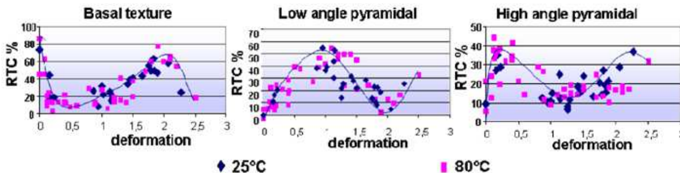
Fig. 7 - RTC of NSK sample as a function of plane-strain deformation rate.
