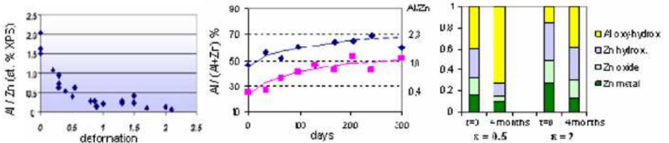
Fig. 9 – Al/Zn XPS ratio as a function of deformation on the left, after ageing for two \epsilon levels on the centre, and Al oxide rebuilding at the expenses of Zn oxide and hydroxide on the right.
