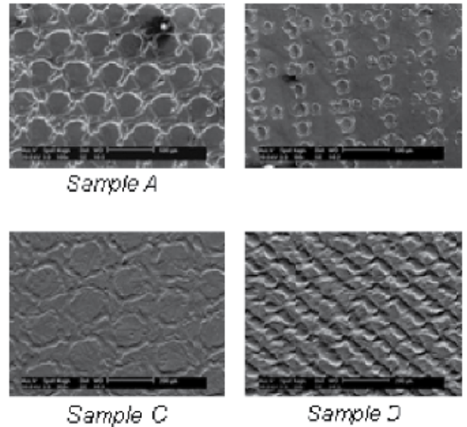
Fig. 1 - Sketch of roughness indentation during skin-pass, with definition of "inter-plateaus", "plateaus" and "valleys" areas and SEM pictures of skin-passed samples.
