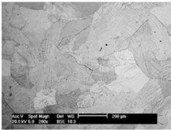
Fig. 3 - SEM picture of NSK GI coating surface (left); Relative Texture Coefficient (RTC) of NSK GI coating, calculated by comparing XRD intensities recorded on coating to the ones recorded on zinc powder (right).
