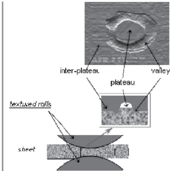
Fig. 1 - Sketch of roughness indentation during skin-pass, with definition of "inter-plateaus", "plateaus" and "valleys" areas and SEM pictures of skin-passed samples.
