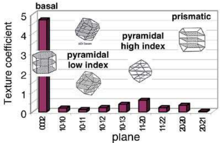
Fig. 3 - SEM picture of NSK GI coating surface (left); Relative Texture Coefficient (RTC) of NSK GI coating, calculated by comparing XRD intensities recorded on coating to the ones recorded on zinc powder (right).
