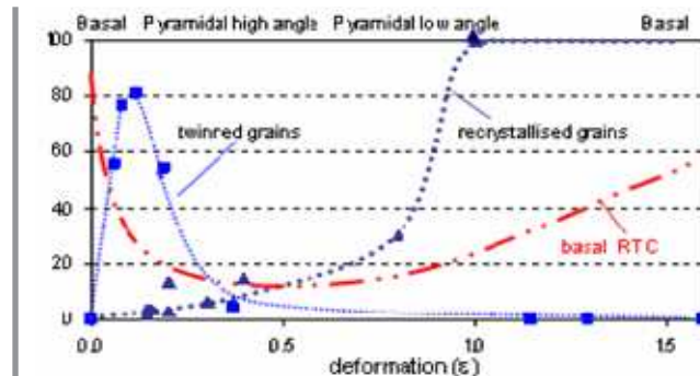
Fig. 8 - Rates of twinned and recrystallized Zn grains as a function of plane-strain deformation rate (sample NSK).
