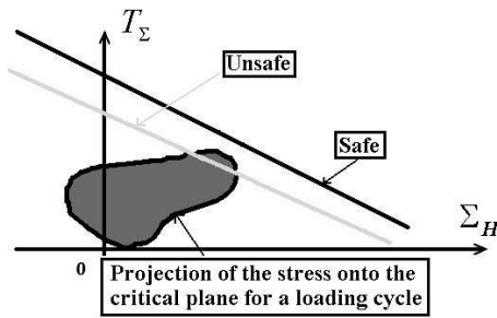
Figure 5: Threshold domain for a determinist fatigue criterion
