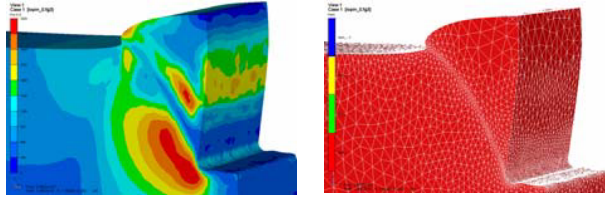
FIGURE 9. Von Mises stress distribution and corresponding mesh at the establishment of the first ASB.
