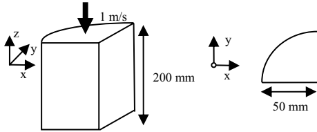
FIGURE 2. Hot Compression test performed on \frac{1}{4} of a cylindrical sample at 1 m/s.
