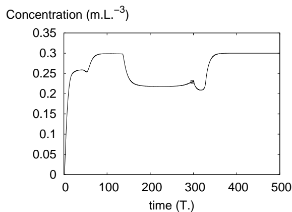
Fig. 13 Elution curve of total dissolved concentration C_3 at x = 2.1L for the dispersive 1D easy test case with n_x = 672 cells.
