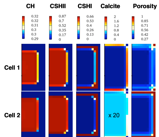
Figure 3: Concentration profiles (in \text{kg}/\text{dm}^3 ) and porosity after 30 days.
