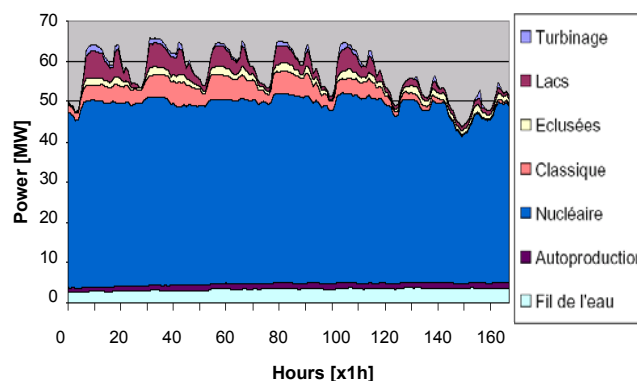
Figure 9 : Example of generation mix for covering the load of one week [13].
