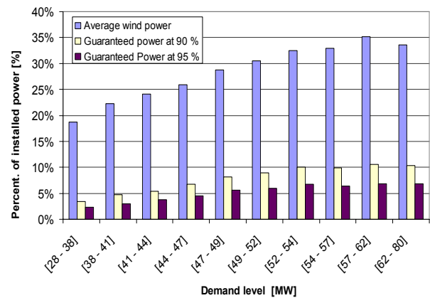
Figure 6: Wind production statistics computed as a function of load level.
