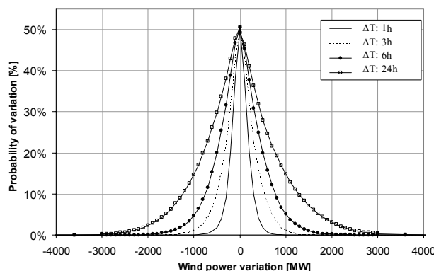
Figure 8: Variations of the hourly wind production corrected for daily trend.
