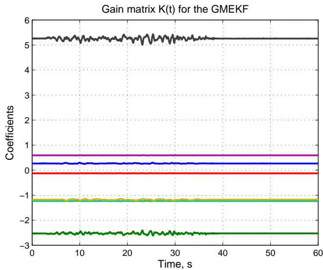
Figure 6. Experiment: Evolution of gain matrix K
