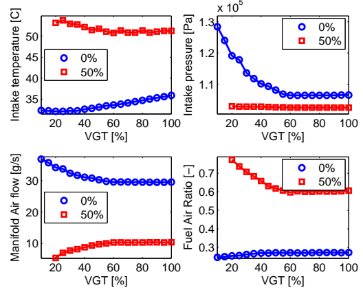
Figure 3. Experimental variation of the VGT actuator at fixed operating conditions (4 bar IMEP injection strategy, N_e = 1500 rpm, EGR valve = 0% and 50%). Effect on the air path.
