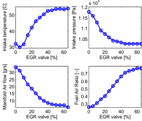
Figure 2. Experimental variation of the EGR valve at fixed operating conditions (4 bar IMEP injection strategy, N_e = 1500 rpm, VGT = 20%). Effect on the air path.
