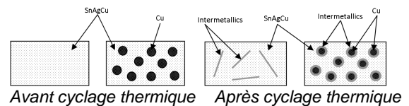
Fig.2: SnAgCu Matrix reinforced by Cu
