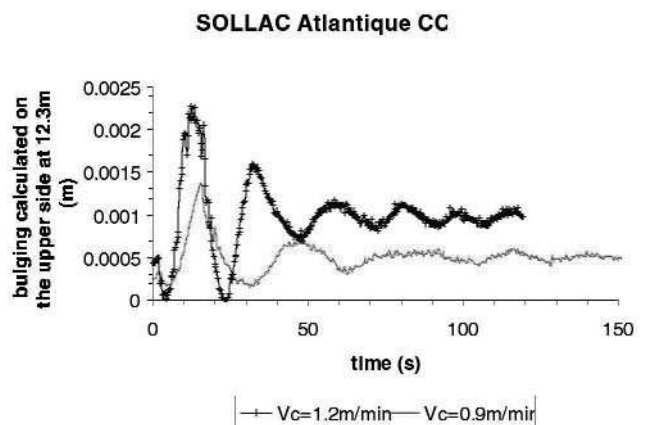
Fig. 8 – The calculated slab bulging converges quickly to a steady state value. It proves the accuracy of the global, non-steady state approach.
