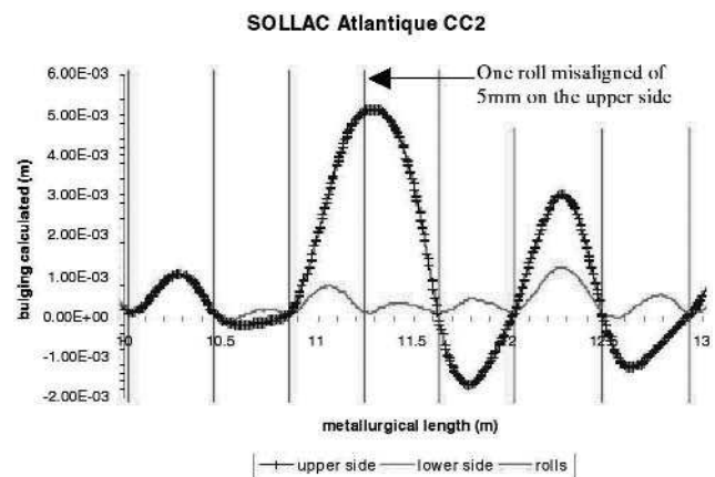
Fig. 10 – A roll misalignment strongly disturbs the bulging profile in following roll pitches.
