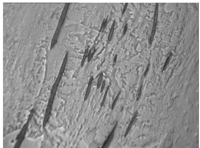
Figure 1. Example of a MnS cluster (S.E.M.)
