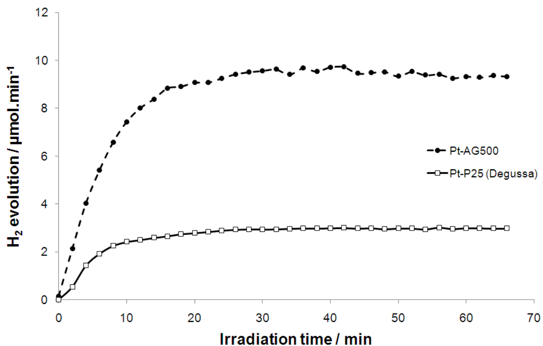
Fig. 19. H 2 evolution on TiO 2 Pt loaded samples : aerogel calcined at 500 °C and P25 - 150 W metal halide lamp, 0.9 l water + 0.1 l MeOH, 0.7 g samples, 0.3 wt% Pt/TiO 2 , room temperature – Strasbourg, France.
