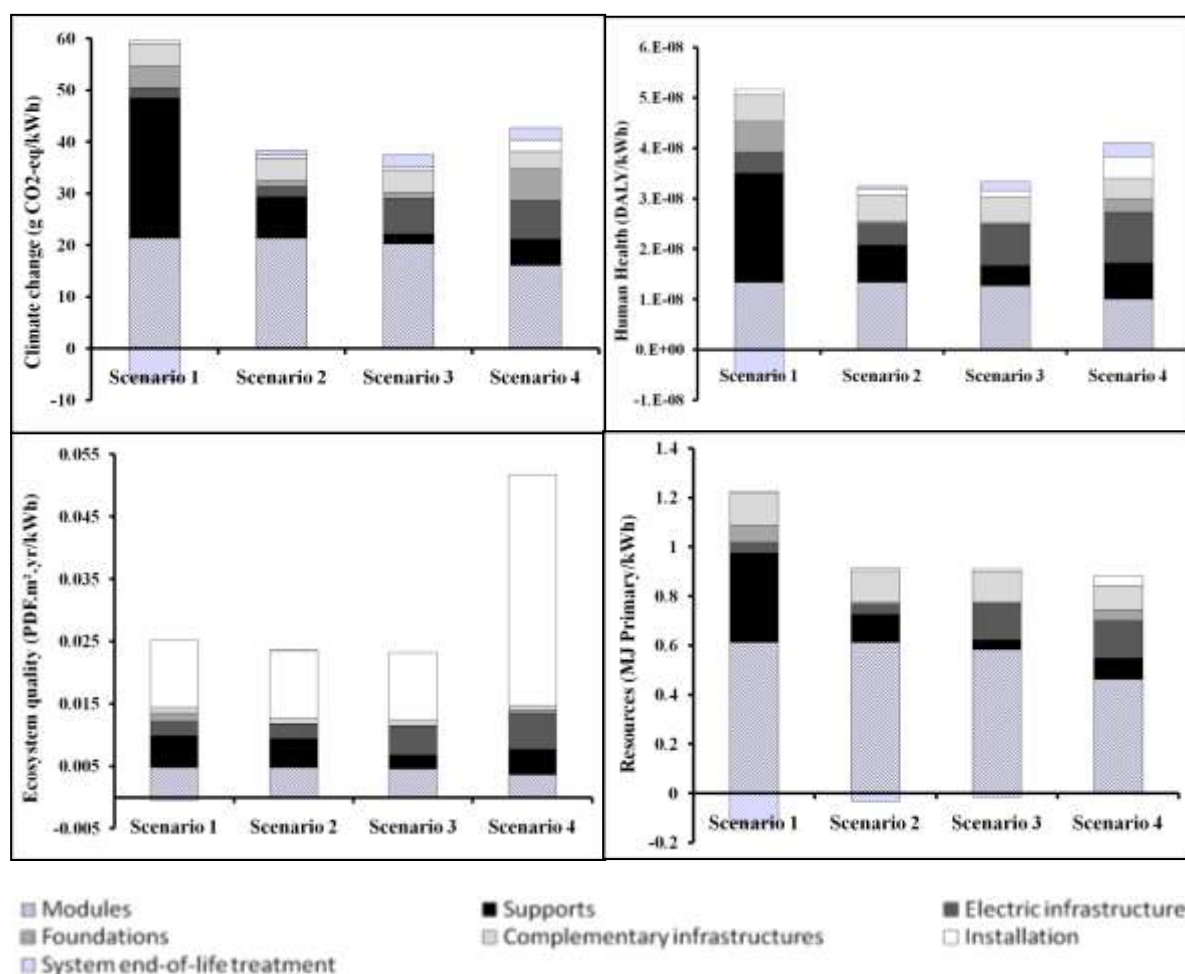
Fig. 2. Detailed environmental impacts of the 4 scenarios (considering 1700 kWh/m 2 .yr of irradiation on an inclined plane, mc-Si modules with 14% of energy production performance and IMPACT2002+v2.04 damage indicators)
