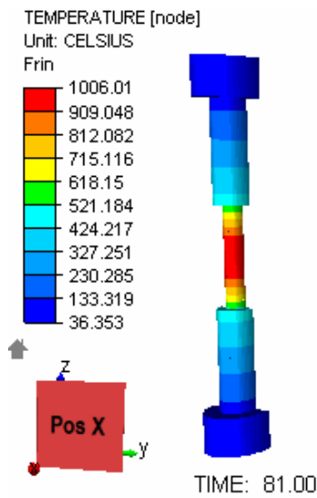
Figure 6. Temperature field (°C) along an axi-symmetric sample.
