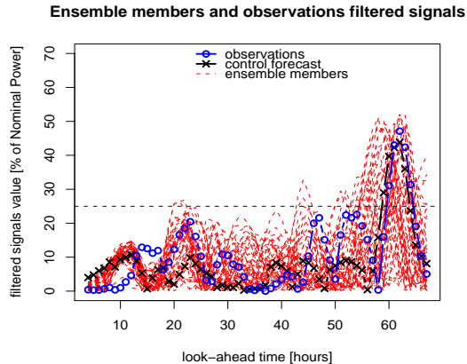
Figure 5: Here is an example of absolute value of filtered signals of observations (blue curve) and ensemble members (red curves, black curve is the control forecast). The ramp observed at horizon 63 is predicted by 39 members, which filtered signals cross over the horizontal dashed line representing the threshold \tau . The resulting timing estimation \bar{h} is equal to 61.
