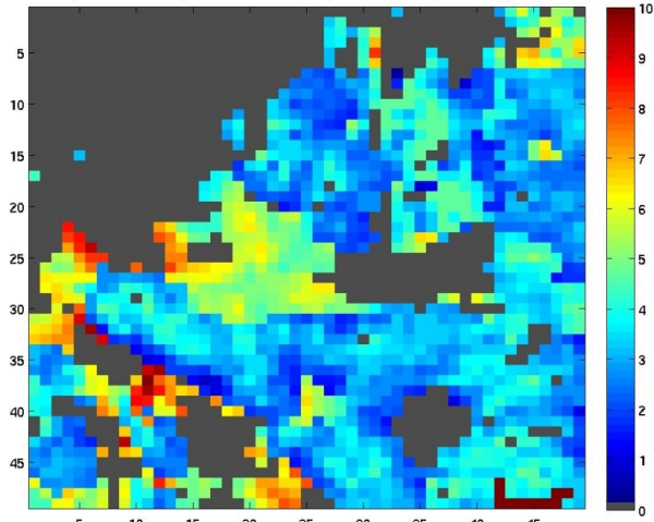
Figure 6: Cloud optical depth from APOLLO (left) and OCA (right) for 3 rd January 2008. 49x49 pixels centered around the station Sede Boqer (position: line 25, column 25)
