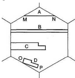
Fig .3, Four morphologies of annealing twins in 2D [14]
