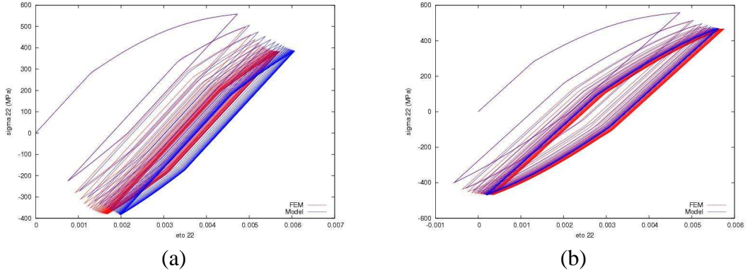
Figure 4: Comparison of the local \sigma_2 - \epsilon_2 histories obtained by FEA and the simplified model for a tension loading: (a) R=0 ; (b) R=-0.3
