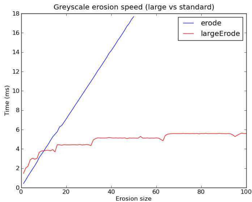
Figure 14: Respective computation times for classical hexagonal erosions (in blue) and for large hexagonal ones (in red). The top chart compares binary operations and the bottom one, 8-bits erosions. Times are given in milliseconds. The image size is 768x576 pixels. These tests have been made with a Core 2 Duo 8400 Intel processor, 3 GHz clock, 4 Go RAM memory running on Linux Fedora 13, 64 bits, SSE2 instructions set enabled.
