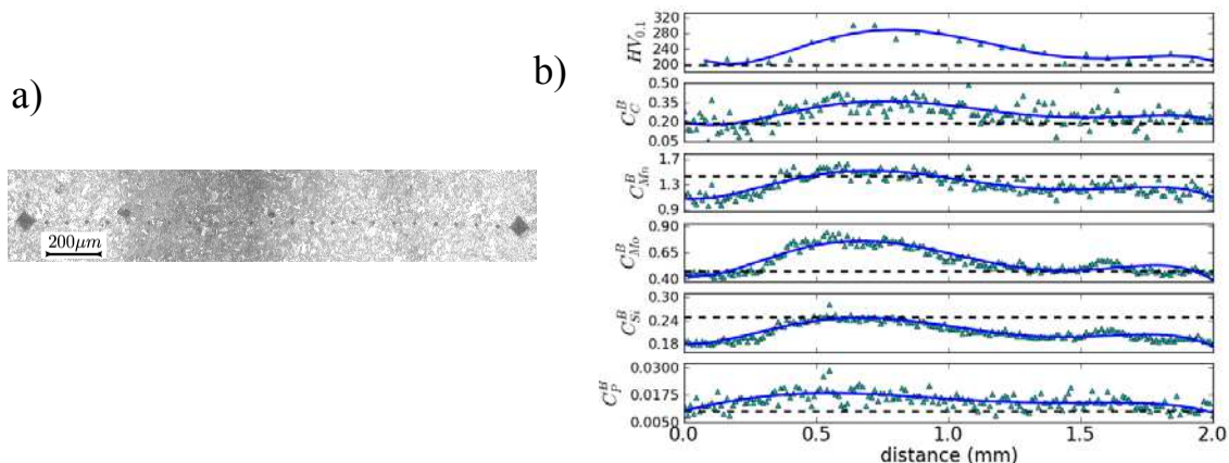
Figure 1. a) Optical micrograph showing two segregated zones aligned along the rolling direction; b) Microprobe analysis across one segregated zone showing the bulk concentration C^B in carbon, manganese, molybdenum, silicon and phosphorus. The variations of micro-hardness (100g) are also shown.
