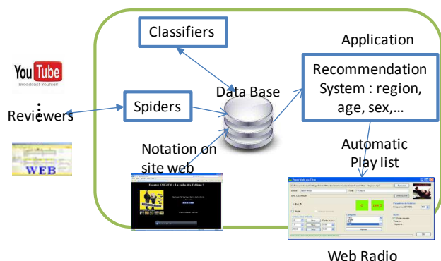
Figure 1: Application architecture.
