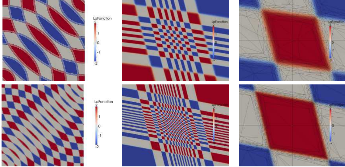
Figure 3: Anisotropic mesh adaptation around the test function f(x) = g \circ g(\|x - 0\|) + g \circ g(\|x - 1\|) with g(x) = \tanh(E \sin(\frac{4*N+1}{2}\pi x)) with 2 sets of parameters : on the top N=3, E=16 and at the bottom N = 6, E = 16 . For these two sets we present : the function on the unit square, one cross detail and a zoom on the mesh for a deep detail inside the cross detail. The 2d adapted meshes containing respectively 1 million and 23 millions nodes. They were built in respectively 576 seconds over 128 cores and 3 hours on 256 cores of Jade supercomputer. The smallest mesh size is around respectively 10^{-5} and 10^{-6} .
