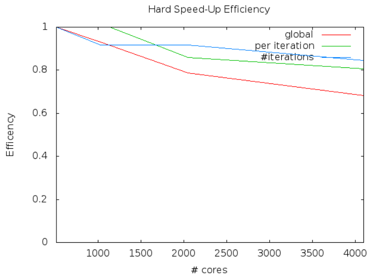
Figure 5: Parallel efficiency for the multigrid resolution using 512 to 4096 cores. The number of multigrid iteration needed to converge stay almost constant (efficiency close to one) has well as the parallel efficiency per iteration. At the global point of view the parallel efficiency is a bit worse due to the combination of per iteration parallel performance and increasing number of iteration but still very good (close to one) has the problem size per core decrease as number of cores used increase.
