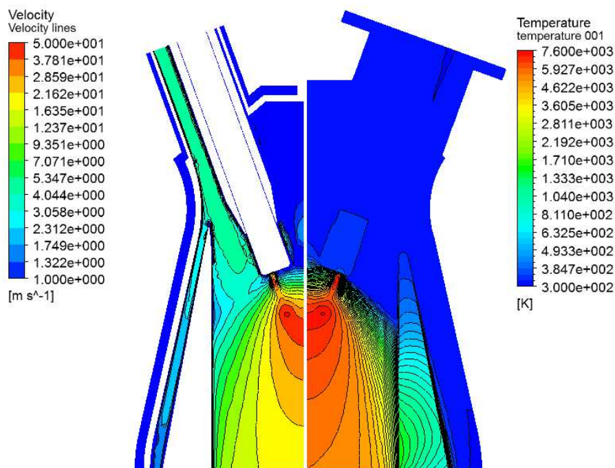
Figure 4: Temperature (right) and velocity (left) fields across the middle plan.
