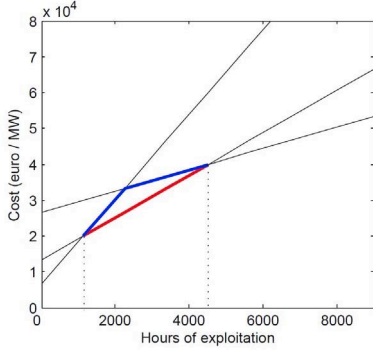
Fig. 3. Minimal (red) and maximal (blue) cost
