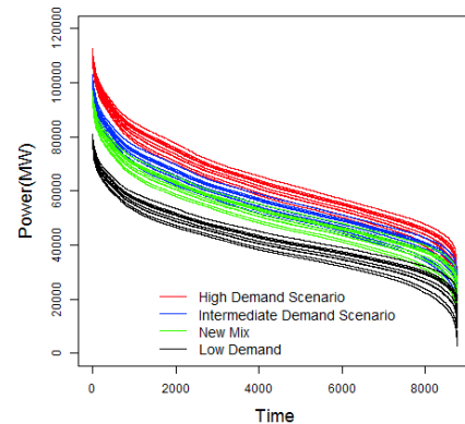
Fig. 4. Load duration curves for each scenario
