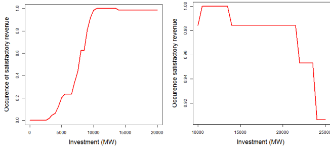
Fig. 9. Probability of satisfying the criterion according to investment levels
