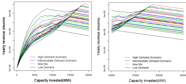
Fig. 8. Benefit according to investment levels for all scenarii
