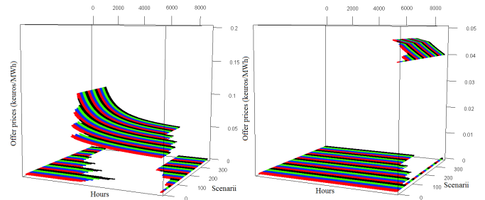
Fig. 6. Offer price for Gas and Coal for all scenarii
