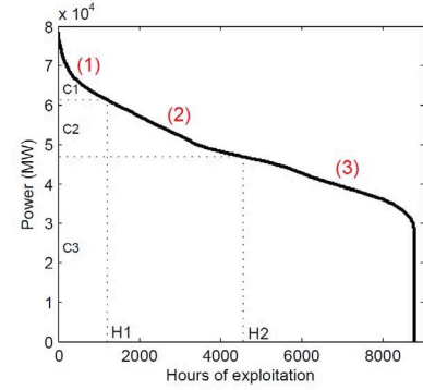
Fig. 2. Example of load duration curve
