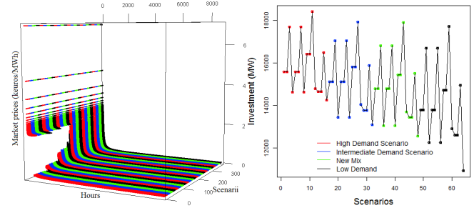
Fig. 7. Market Price and recommended investment per scenario
