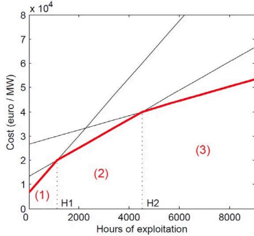
Fig. 1. Example of 3 cost functions
