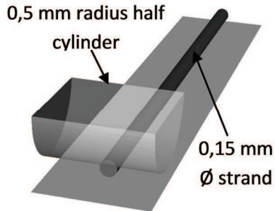
Fig. 4. Strand compression inverse analysis model.
