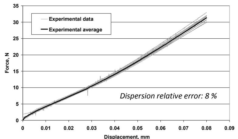
Fig. 2. Experimental results of copper strands compression tests.
