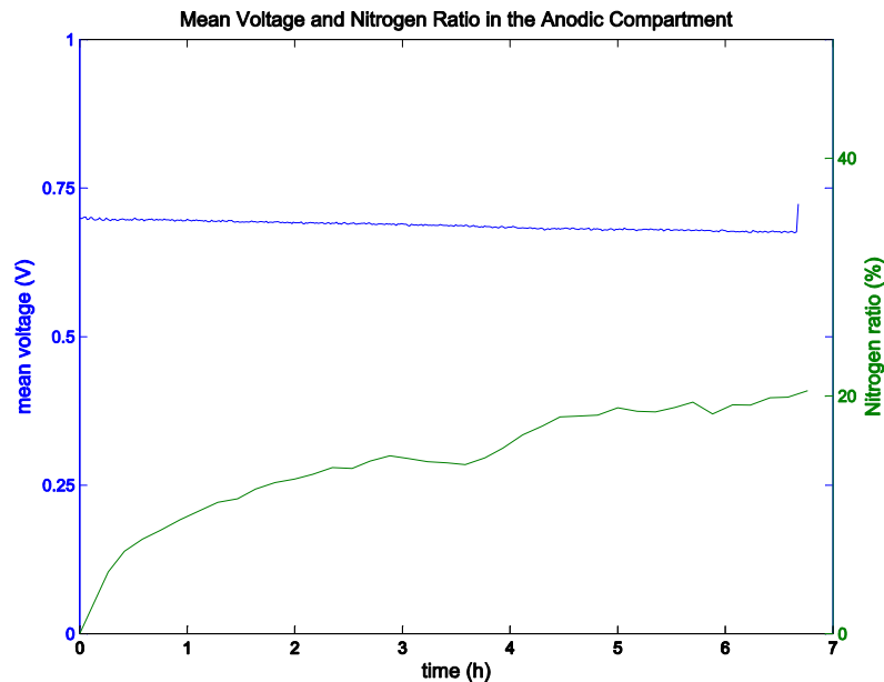
Fig : Mean Voltage and Nitrogen accumulation during a 6h45 long test of the PSR system at 0.5 A/cm 2
