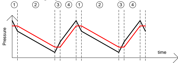
Fig2 : Evolution of pressure in the anodic compartment (black) and the gas tank (red)
