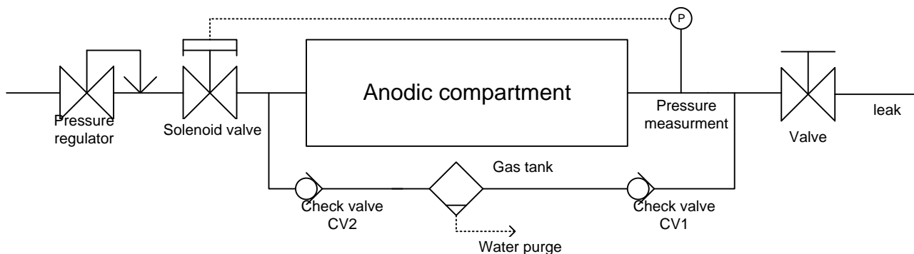
Fig1 : Schematic diagram of the pressure swing recirculation system.
