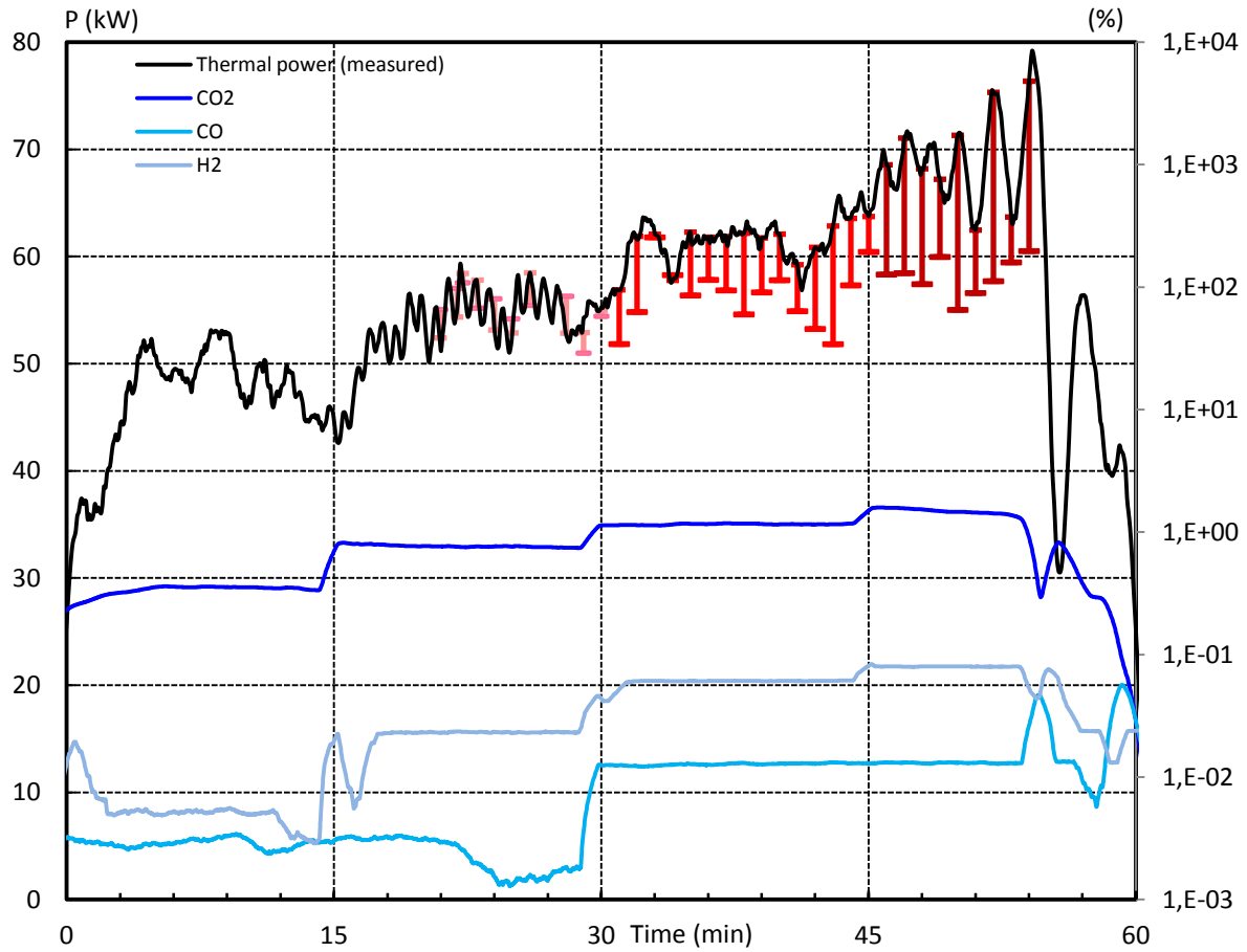
Figure 4: Total measured thermal power (black) , CO 2 , CO and H 2 volume percentage (from dark to light blue). The colored arrows represent the difference between the total measured thermal power and the measured electric power at different biomass injection rate 1.1 kg.h -1 , 2.2 kg.h -1 and 3.3 kg.h -1 (from light to dark red).
