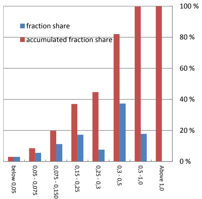
Figure 1: Mass distribution of biomass granulometry (dimension in mm).
