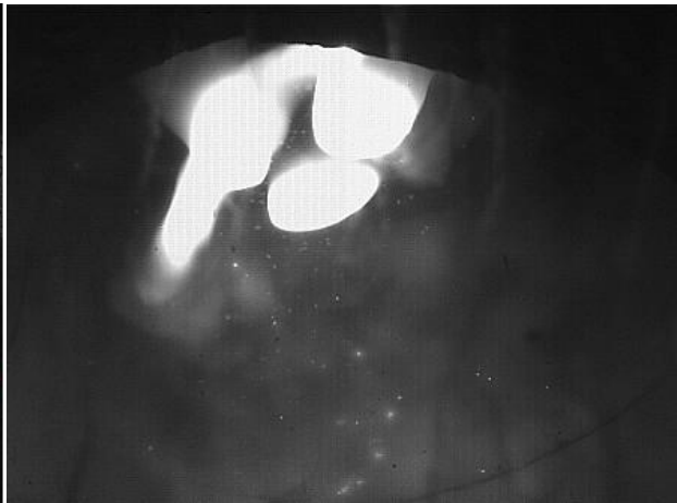
Figure 6: Shot of the arc discharge zone (electrode, electric arc and burning biomass particle) the feeding rate is 1 \text{ kg.h}^{-1} .
