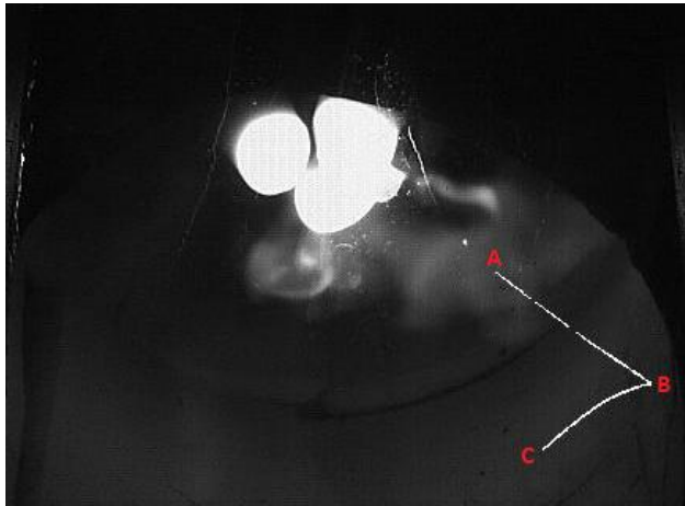
Figure 5: trajectory of a graphite electrode particle during a test without combustion (superposition of 300 frames captured at 150,000 fps)
