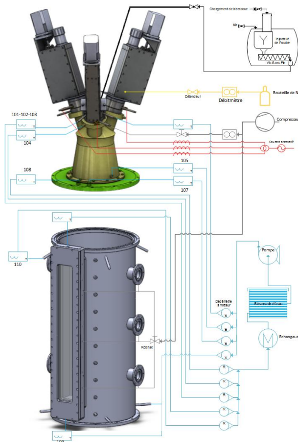
Figure 2 : P&D of the experimental setup (three phase plasma torch (top left) and combustion chamber (bottom left))
