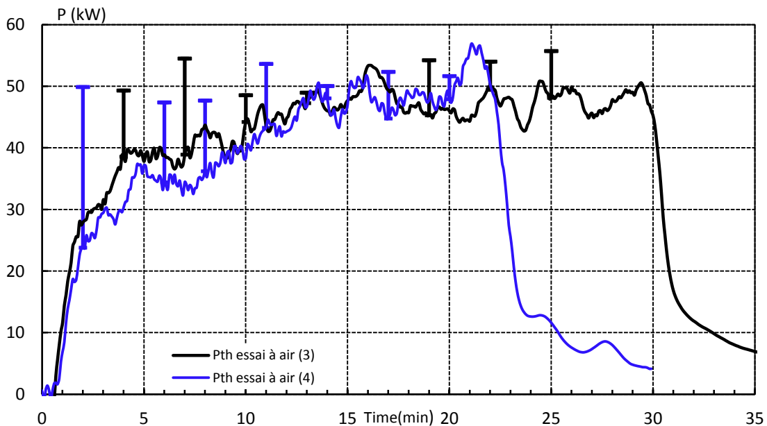
Figure 3: Total measured thermal power of two tests without combustion and the difference with measured electric power.
