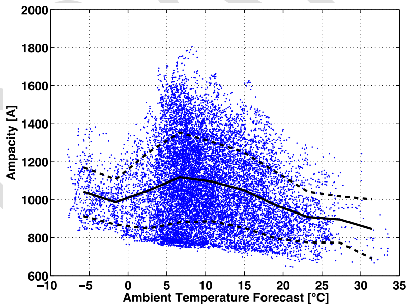
Figure 9: Two-day ahead ambient temperature forecast has a significant influence on ampacity; data from a 150kV line in Belgium, near the North Sea [mean \pm 1 std] (EU funded TWENTIES project, NETFLEX Demo)
