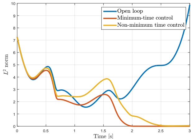
Fig. 1. Time evolution of the L2-norm in open loop and using two different controllers
