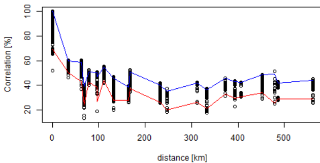
Figure 6: Evolution of correlations between the difference of mean hourly production values, and 5 minutes resolution production values, as a function of the distance between sites.
