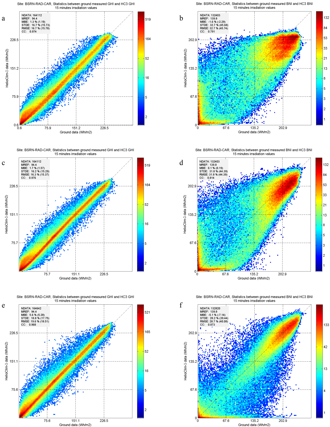
Fig. 2. (a) 2-D histogram of the 15 min HC3v4 GHI values versus the measurements of the BSRN station of Carpentras; (b) HC3v4 BNI; (c) HC3v5 GHI; (d) HC3v5 BNI; (e) MACC-RAD GHI; (f) MACC-RAD BNI
