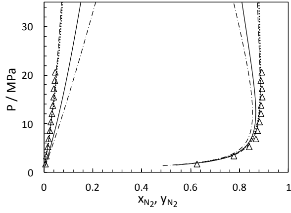
Fig 7. Pressure–composition diagram of the \text{N}_2 + \text{H}_2\text{S} system at 256K. Comparison between experimental data ( \triangle ) [48], the SAFT-VR Mie EoS with k_{ij}=0 (continuous line) and with regressed k_{ij} (dashed lines) and the PR EoS with k_{ij}=0 (dot-dashed line) and with regressed k_{ij} (dotted line).
