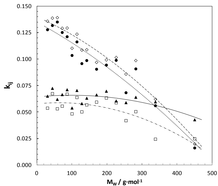
Figure 3. Binary interaction parameters of n -alkanes + CO_2 binary system and their trend curves for the SRK ( \diamond , dashed lines), PR ( \bullet , dotted line), PC-SAFT ( \blacktriangle , continuous line) and SAFT-VR Mie ( \square , dot-dashed line) EoS.
