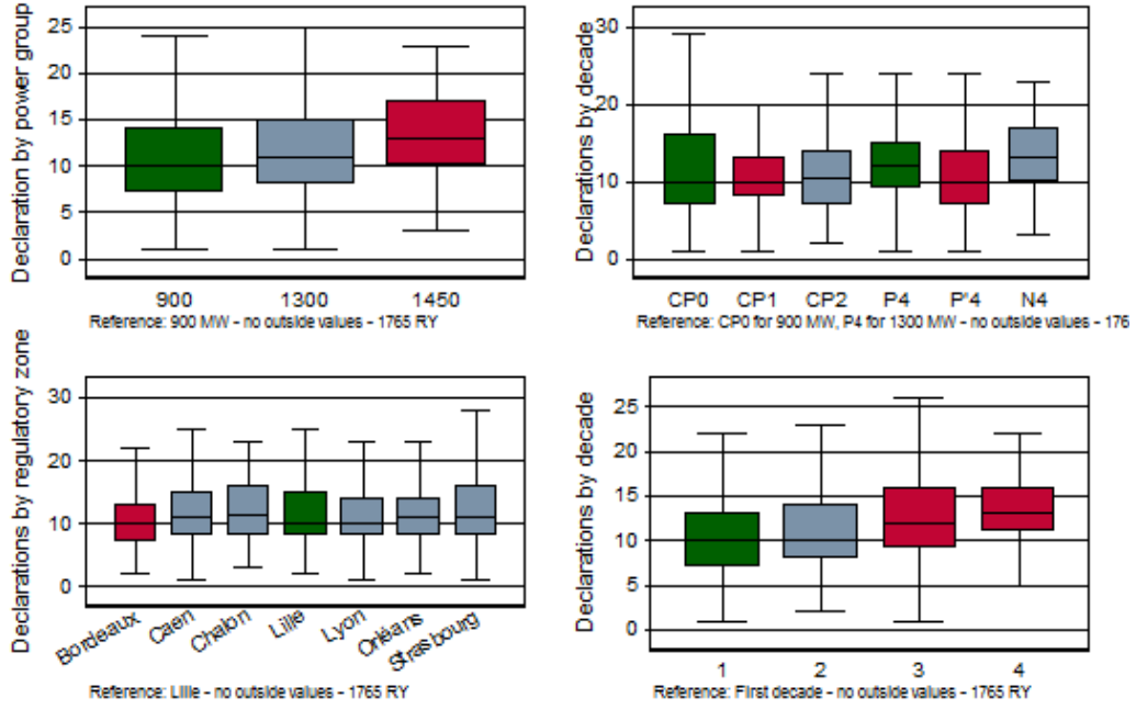
Figure 2: Annual declarations by reactor for different groups of reactors
