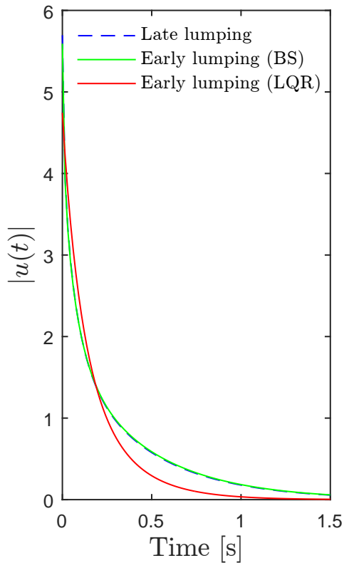
Control effort
