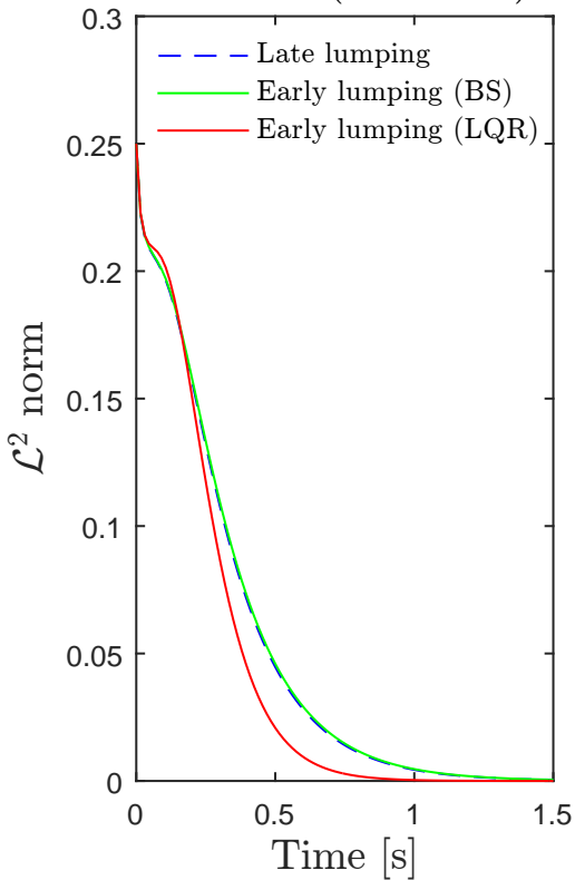
\mathcal{L}^2 -norm (30 modes)
