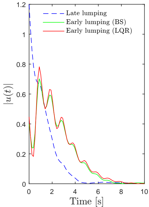
Control effort
