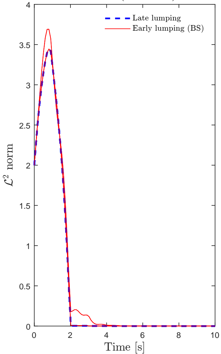
\mathcal{L}^2 -norm (10 modes)
