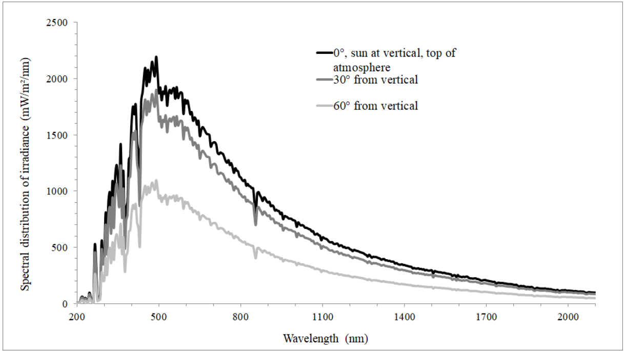
Figure 5.2. Typical spectral distributions of the solar irradiance received by a horizontal surface at the top of the atmosphere for wavelengths from 200 nm to 2000 nm for three solar zenithal angles: 0°, 30°, and 60°.
