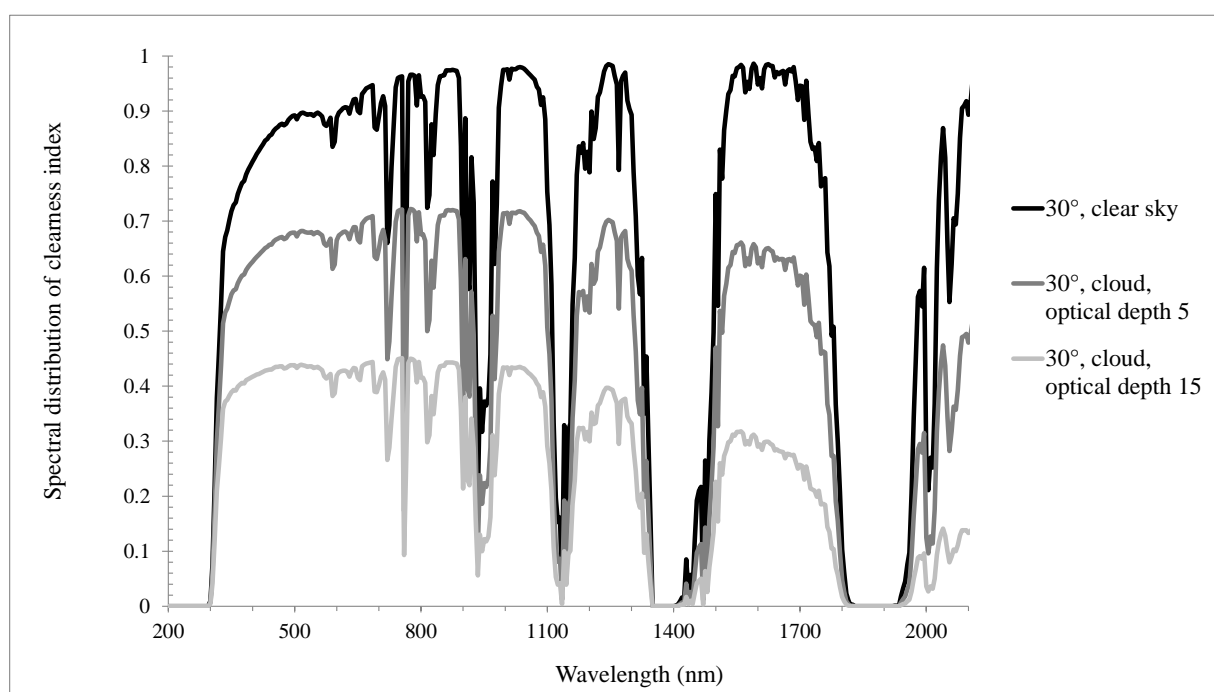
Figure 6.8. Typical spectral distribution of clearness index for wavelengths from 200 nm to 2000 nm for a solar zenithal angle of 30°. The surface is horizontal at ground level. Clear sky conditions (visibility of 50 km, black line) and cloudy conditions with two optical depths: 5 (dark grey line) and 15 (light grey line).
